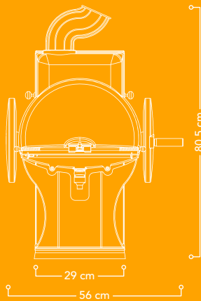
vista frontal
