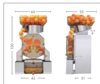
Citrocasa 8000 XB with Juice-Tank Art.-No. 80.002
