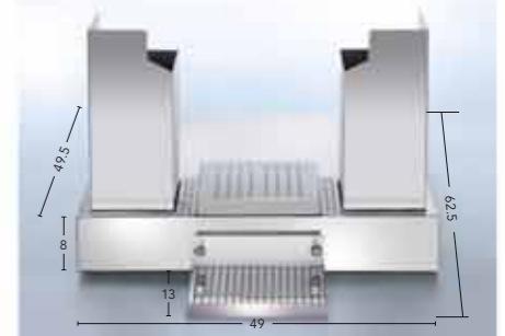
Counter top installation kit 6000/7000 Art.-No. 70.878
